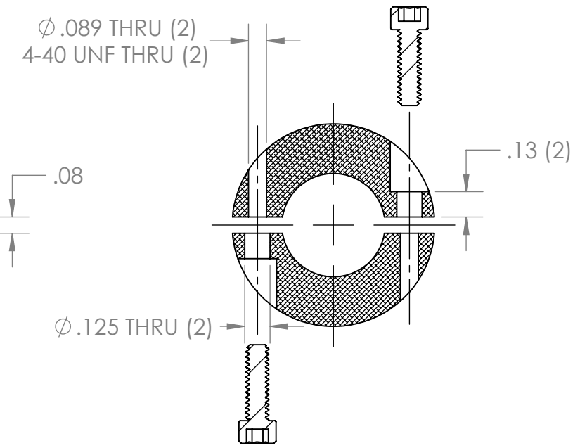
SECTION B-B
